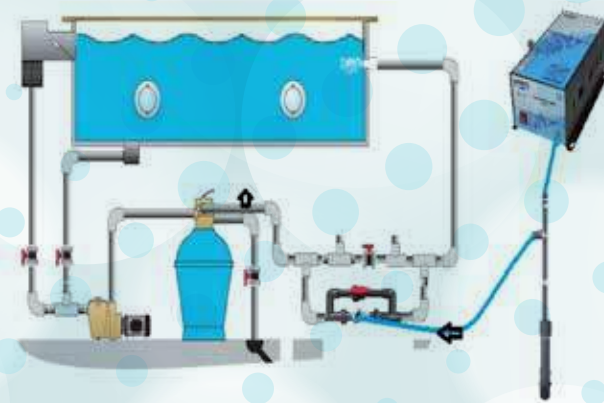
VENTURI FOR DOMESTIC POOLS BY-PASS INSTALLATION DIAGRAM
