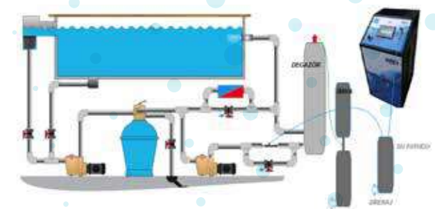
DOZON MAXI DEGASTOR ASSEMBLY DIAGRAM
