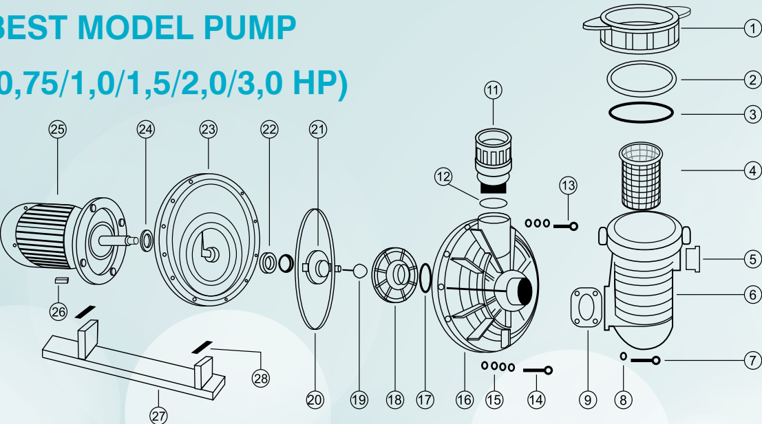
Atlaspool Pool Pumps Spare Parts List
