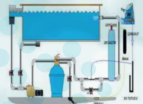
DOZON MIDI DEGASTORS INSTALLATION DIAGRAM
