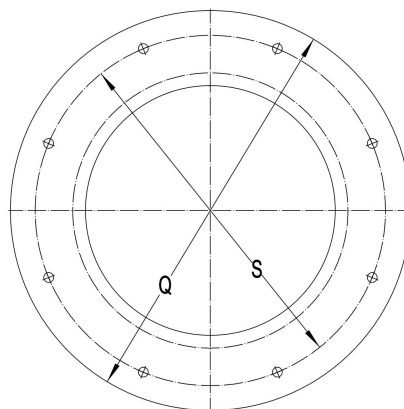
MOUNTING FLANGE
