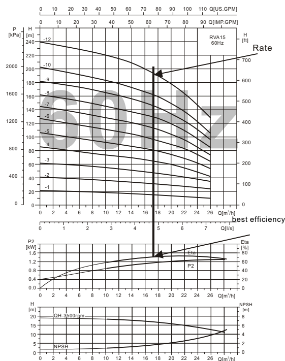
Fig.6 example of duty point
