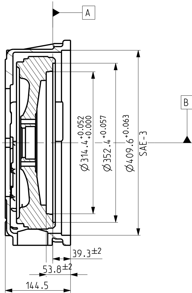
FLYWHEEL END DETAIL
