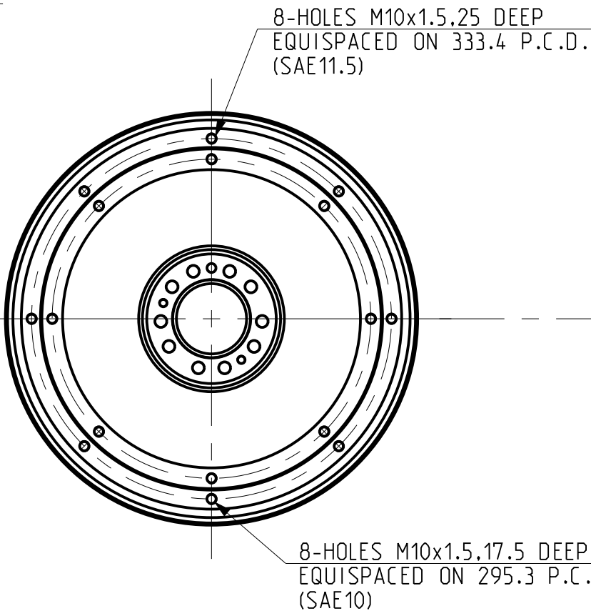
FLYWHEEL END DETAIL
