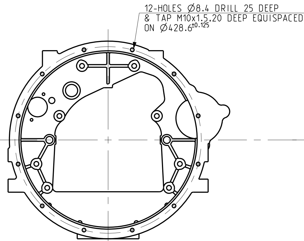
FLYWHEEL HOUSING
