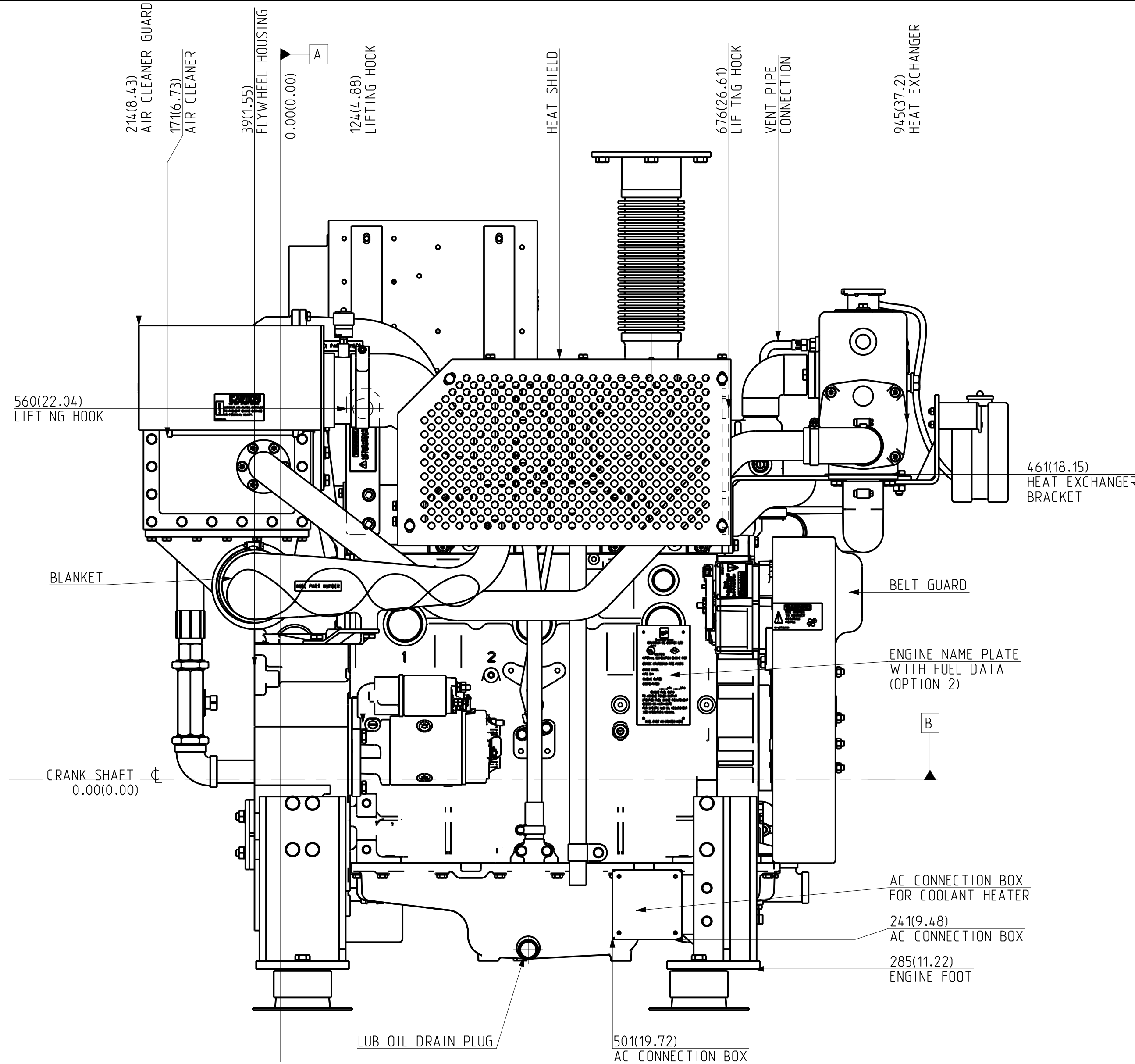
VIEW FROM EXHAUST SIDE
