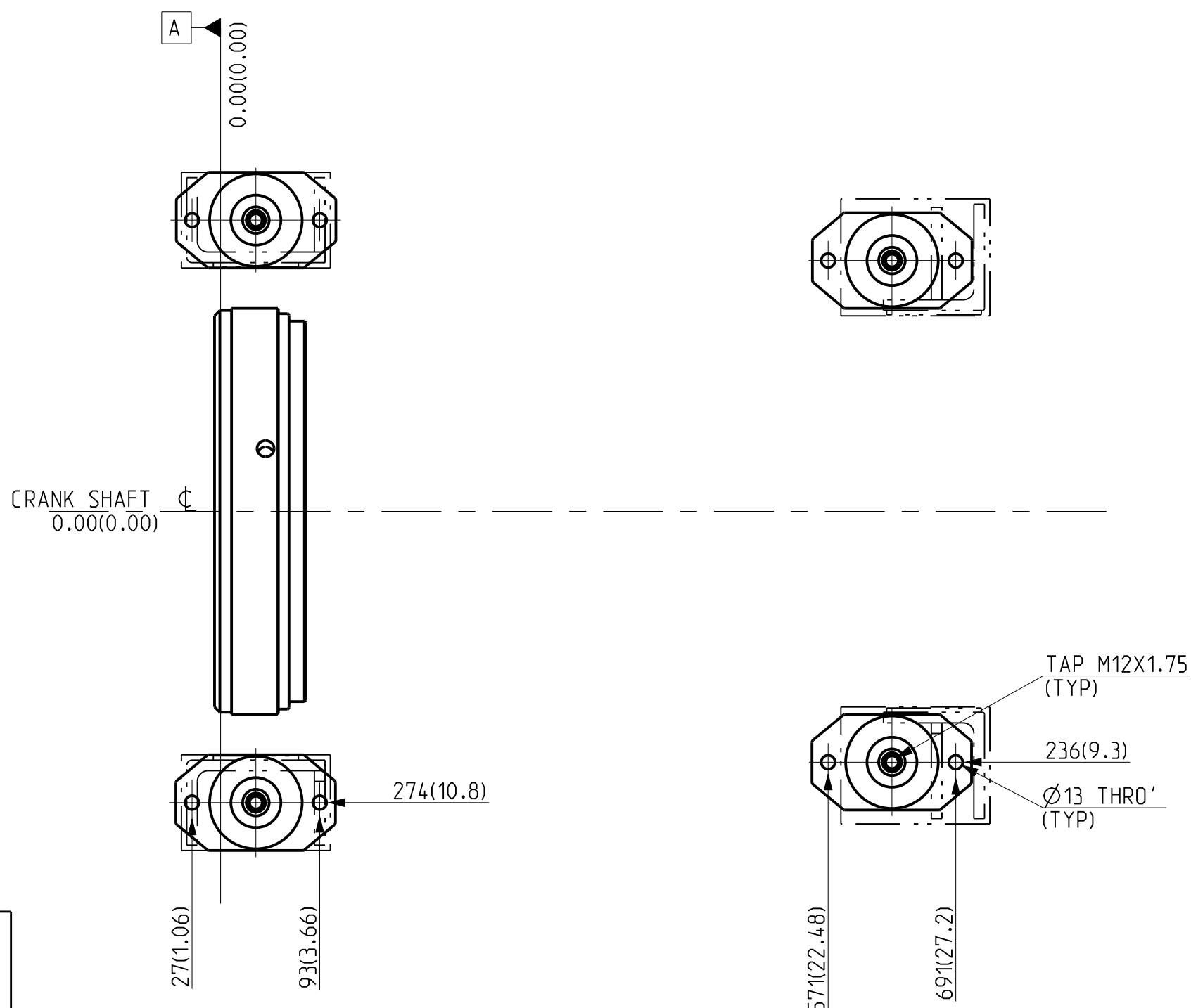
FOUNDATION PLAN VIEW
