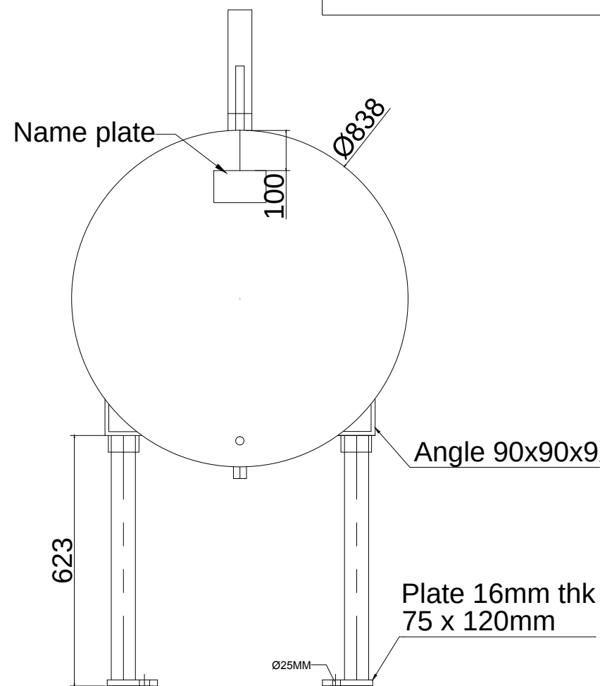
tank side view
