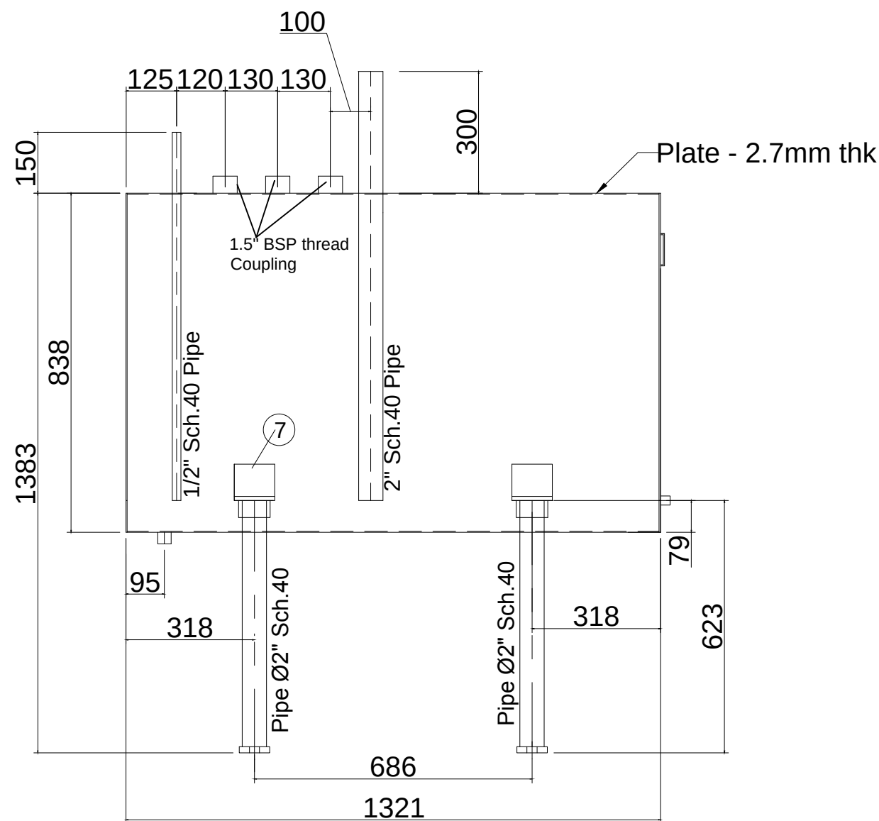
tank front view
