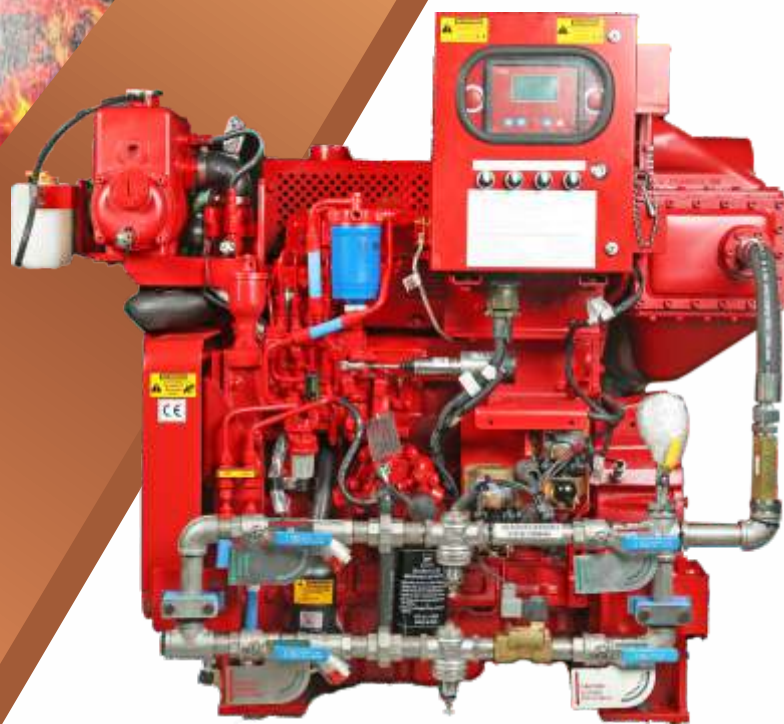
Diesel Engines for Fire Pumps
